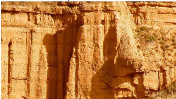
Badlands in Spain
